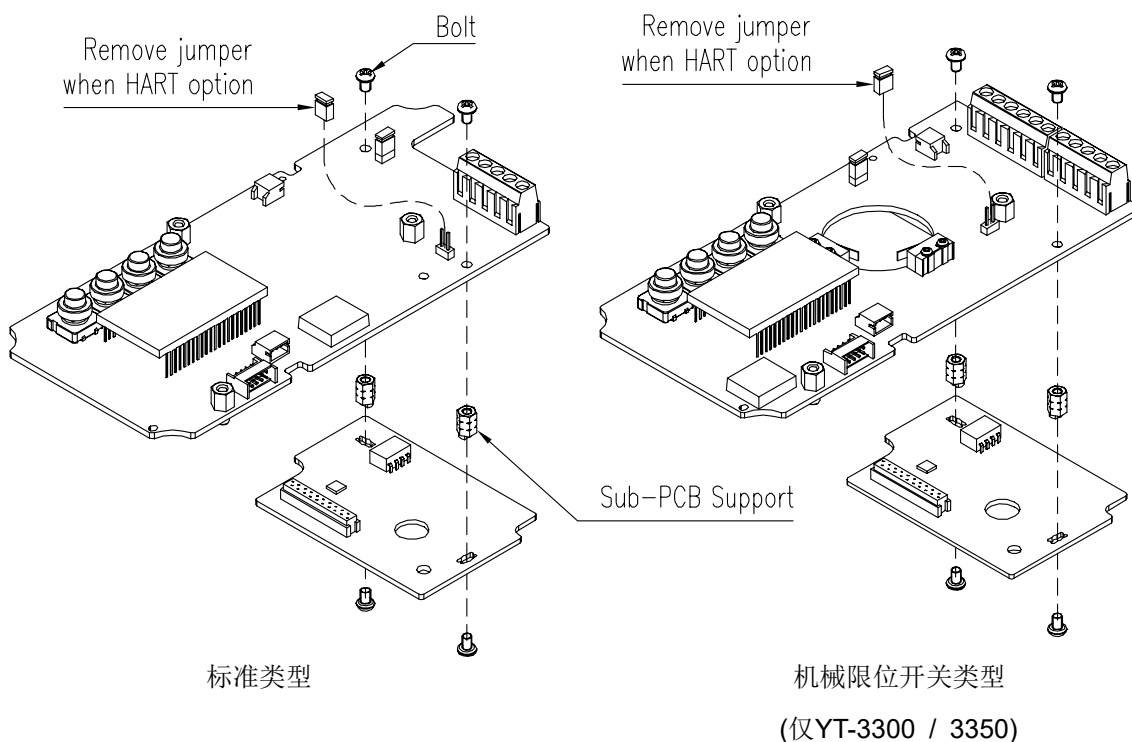
图7-2: 将选配型PCB安装于主PCB上
